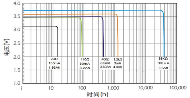
2. Voltage curve under different current and temprature (Stable discharge process)
