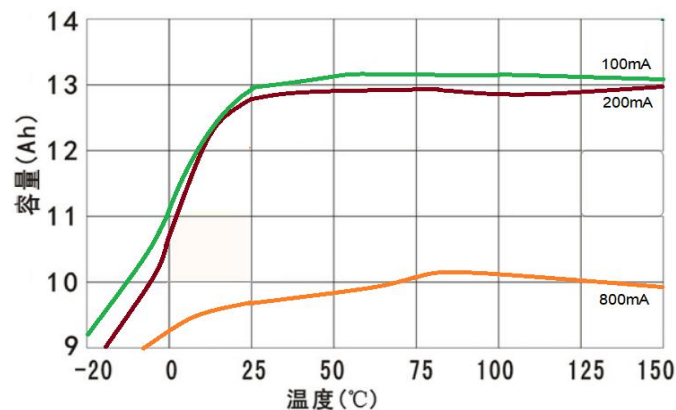
3. Capacity curve under different temperture and current (cutoff voltage 2.0V)
